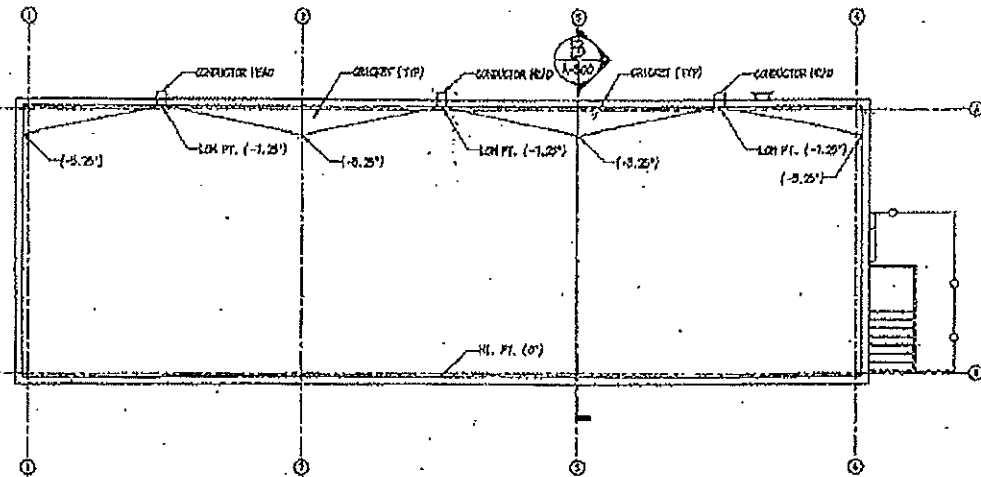
C ROOF PLAN A-101 SCALE: 1/8" = 1'-0" PROJECT NORTH
