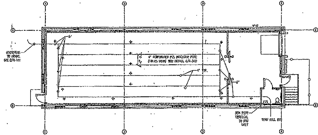
D UNDER SLAB VENTILATION PLAN A-101 SCALE: 1/8" = 1'-0" PROJECT NORTH
