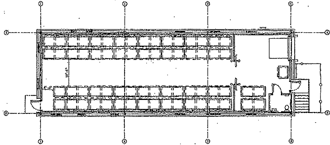
B RACKING PLAN A-101 SCALE: 1/8" = 1'-0" PROJECT NORTH
